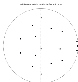
Figure C1. Inverse Roots of AR Characteristic Polynomial
